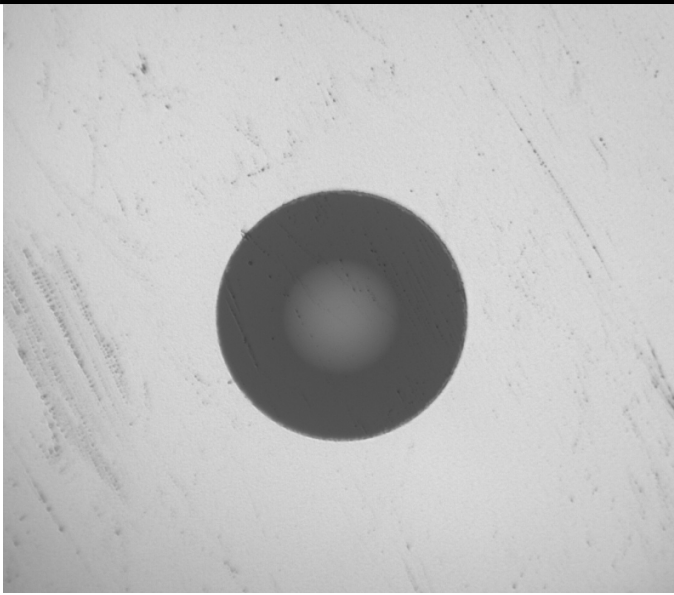
Input Image
