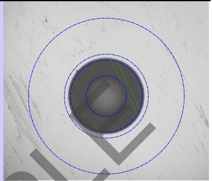
Analysis Image
